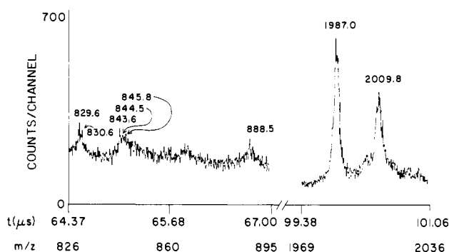
Figure 1. Portions of positive ion time-of-flight spectrum of synthetic alamethicin I. Reproduction of computer graphic output. Left display: portion of fragmentation region; right display: quasi-molecular ion region.
